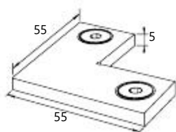
Connector 90° for F50-201 handrail
