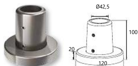
Heavy duty support foot for Ø42 column Κωδ. / Code 4127 Συσκ. / Pack. 20 τεμ./pcs.
