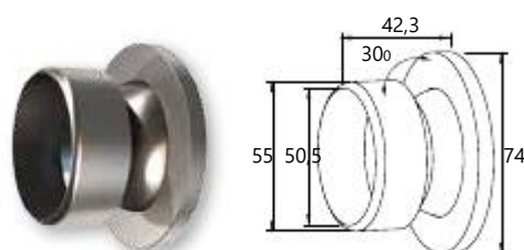
Wall cover for handrail Ø50 with cap Κωδ. / Code 4518 Συσκ. / Pack. 20 τεμ./pcs.
