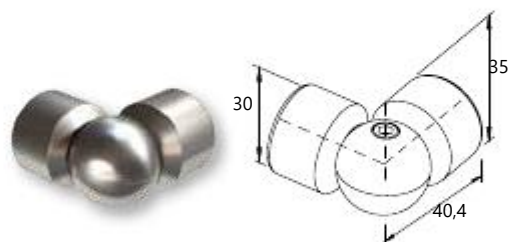
Adjustable corner connector for F50-307 guide
