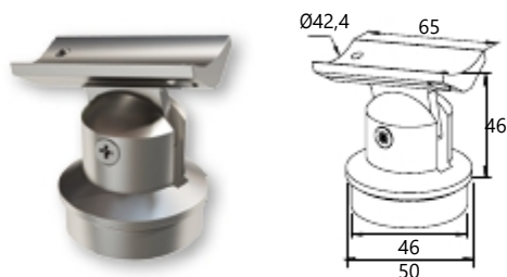
Connector for F50-100 column with F50-200 handrail
