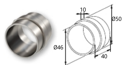
Connector for handrail Ø50 (internal)
