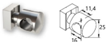
Connector for profile Ø16 with BLADE column
