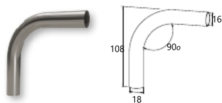
Connector 90° for profile Ø16
