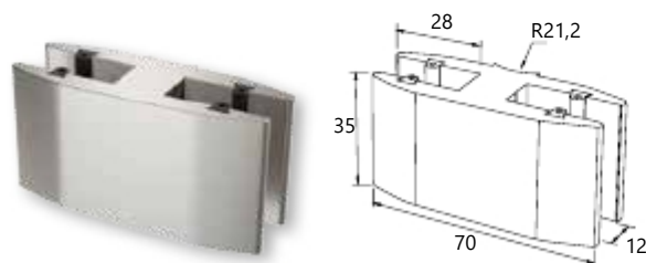
Double glass support 8-10 mm for F50-103 column
