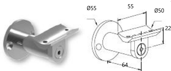
Wall support for F50-200 handrail Κωδ. / Code 4140 Συσκ. / Pack. 20 τεμ./pcs.
