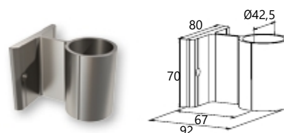
External support for Ø42 column Κωδ. / Code 4166 Συσκ. / Pack. 10 τεμ./pcs.
