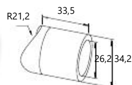
Connector for F50-100 Column with profile Ø26
