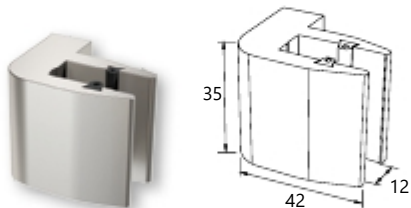
Single glass support 8-10 mm for F50-102 column
