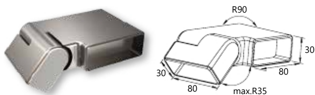
Adjustable corner connector 90° for 80x30 handrail (stairs)
