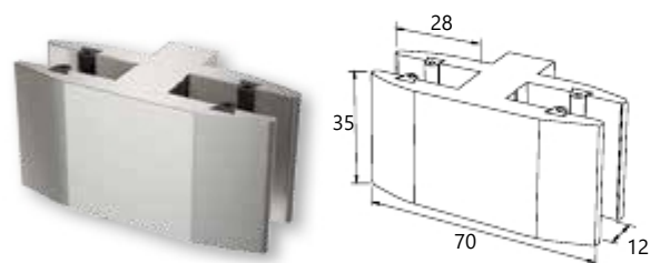
Double glass support 8-10 mm for F50-102 column
