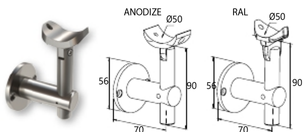
Wall support for F50-200 handrail Κωδ. / Code 4165 Συσκ. / Pack. 20 τεμ./pcs.
