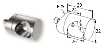
Connector for F50-101 column with profile Ø26
