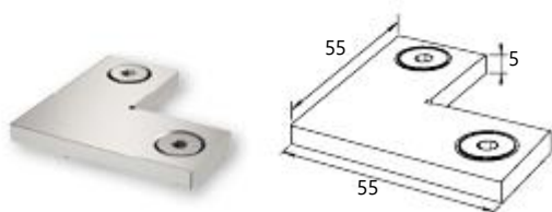
Connector 90° for F50-201 handrail
