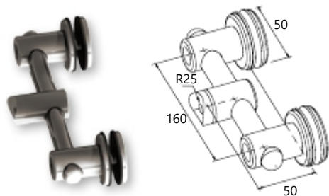
Double glass support 8-10 mm for Ø50 column
