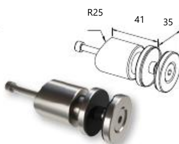
Glass support 8-10mm for F50-101 column Κωδ. / Code 4137 Συσκ. / Pack. 10 τεμ./pcs.
