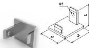
End cap for F50-319 guide
