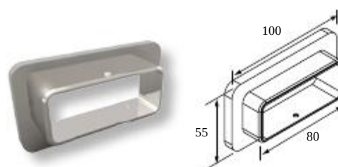
Wall cover for F50-201/203 handrail (with cap) Κωδ. / Code 4515Z Συσκ. / Pack. 40 τεμ./pcs.
