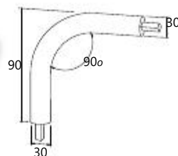
Connector 90° for F50-307 guide
