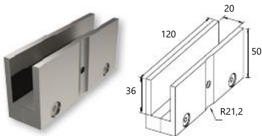
Single glass support 8-10 mm for F50-102/106 columns Κωδ. / Code 4193 Συσκ. / Pack. 50 τεμ./pcs.
