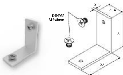
Connector for F50-319 guide
