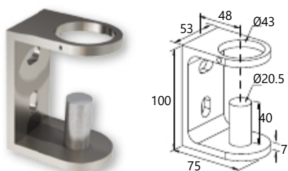
External support for F50-100/103 column Κωδ. / Code 4143 Συσκ. / Pack. 12 τεμ./pcs.
