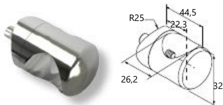
Connector for F50-101 column with profile Ø26
