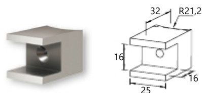
Connector for F50-100 Column with F50-302 profile
