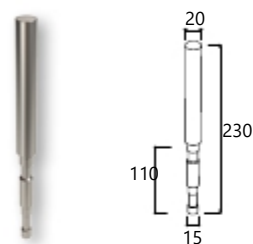
Infloor support for F50-102 column
