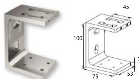
External support for BLADE column Κωδ. / Code 4142 Συσκ. / Pack. 12 τεμ./pcs.
