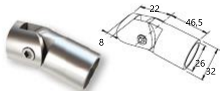
Connector for F50-102 column with profile Ø26
