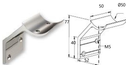
External support for 40x40 column Κωδ. / Code 4139 Συσκ. / Pack. 12 τεμ./pcs.
