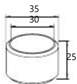
Connector for guide Ø30 (straight)
