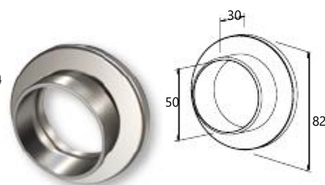
Wall cover for handrail Ø50 with cap Κωδ. / Code 4509Z Συσκ. / Pack. 20 τεμ./pcs.
