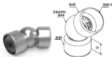
Adjustable corner connector for handrail Ø40
