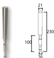
Wall support for F50-200 handrail Κωδ. / Code 4165 Συσκ. / Pack. 20 τεμ./pcs.
