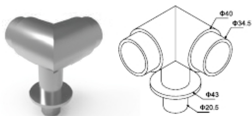
Connector 90° for handrail Ø40
