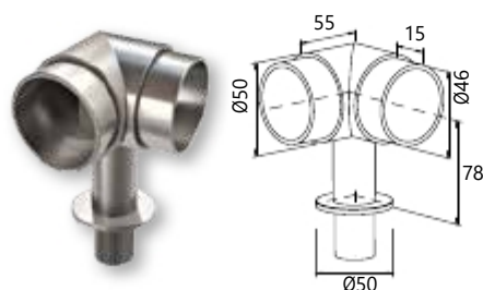
Connector 90° for handrail Ø50
