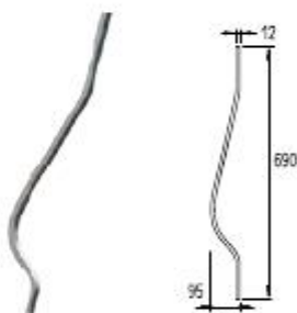
Curved profile for Vertical-D Κωδ. / Code 4670 Συσκ. / Pack. 100 τεμ./pcs.
