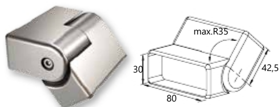
Adjustable corner connector for 80x30 handrail (stairs)
