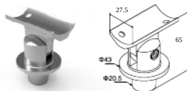
Adjustable corner support for handrail Ø40 - column Ø42
