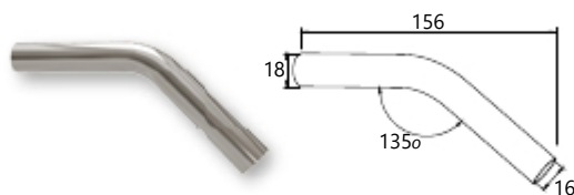
Connector 135° for profile Ø16
