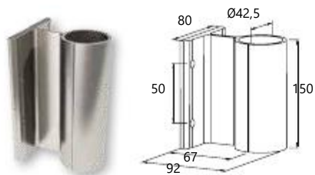
External support for column Ø42 Κωδ. / Code 4194 Συσκ. / Pack. 20 τεμ./pcs.
