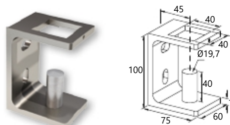
External support for F50-102 column Κωδ. / Code 4144 Συσκ. / Pack. 12 τεμ./pcs.
