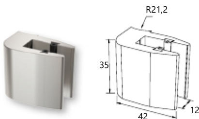
Single glass support 8-10 mm for F50-103 column
