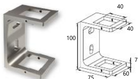
External support for 40x40 column Κωδ. / Code 4139 Συσκ. / Pack. 12 τεμ./pcs.
