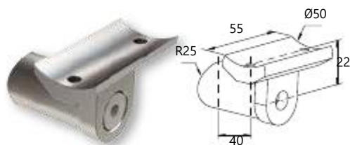
External Support for F50-200 handrail to F50-101 column
