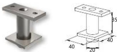
Support for F50-102 column with F50-201 handrail
