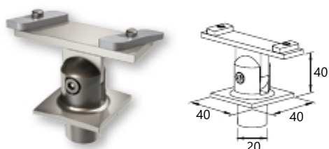
Connector for F50-102 column with F50-201 handrail
