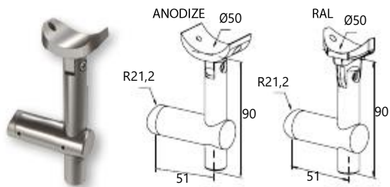
External support for handrail Ø50-column Ø42
