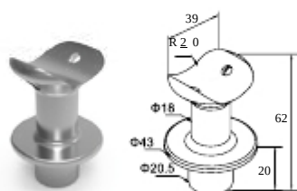
Support for handrail Ø40-column Ø42 (stairs)
