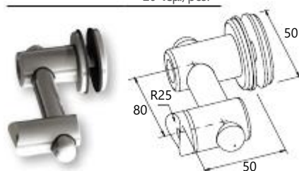
κολώνας F50-101 Support for F50-200 handrail- F50-101 column
