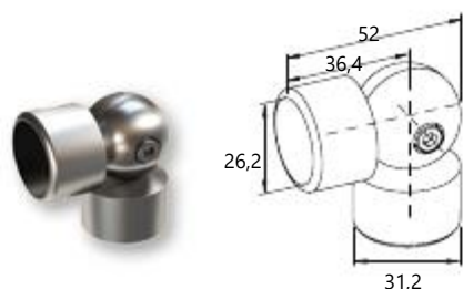
Adjustable corner connector for profile Ø26
