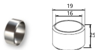
Connector for profile Ø16 (straight)
