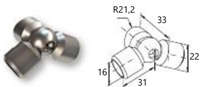
Adjustable corner connector for profile Ø16 with F50-100 column
