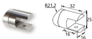
Connector for F50-100 Column with F50-302 profile
