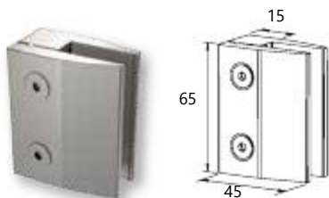
Single glass support 8-10 mm for F50-102/106 columns Κωδ. / Code 4193 Συσκ. / Pack. 50 τεμ./pcs.
