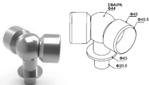
Adjustable corner connector for handrail Ø40 with column Ø42
