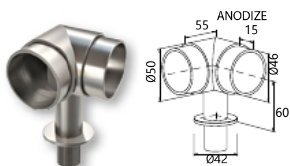
Ø50 Railtop corner Connector 90° for handrail Ø50
