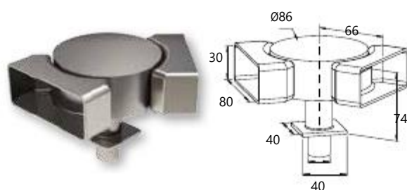
Adjustable corner connector for 80x30 handrail with F50-102 column
